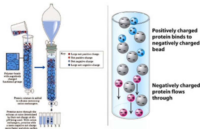
Figure 2: Ion exchange chromatography
