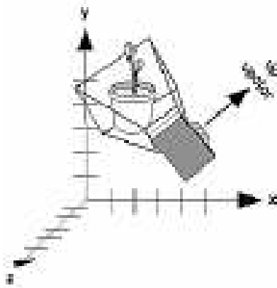
Figure 12 : Using gluLookAt()
