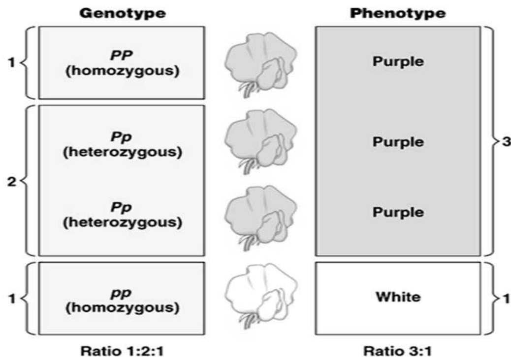
Figure 11.1 Genotype & Phenotype
