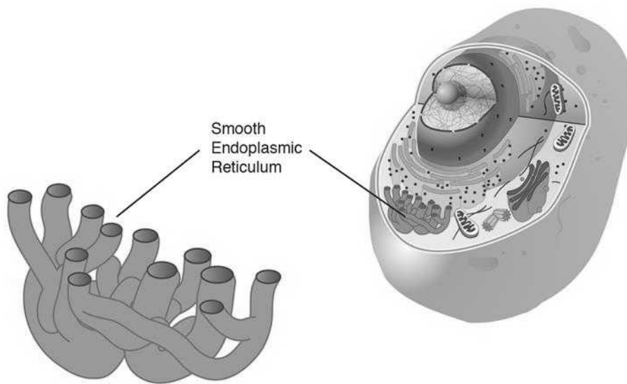
Figure 8.4 Endoplasmic reticulum
