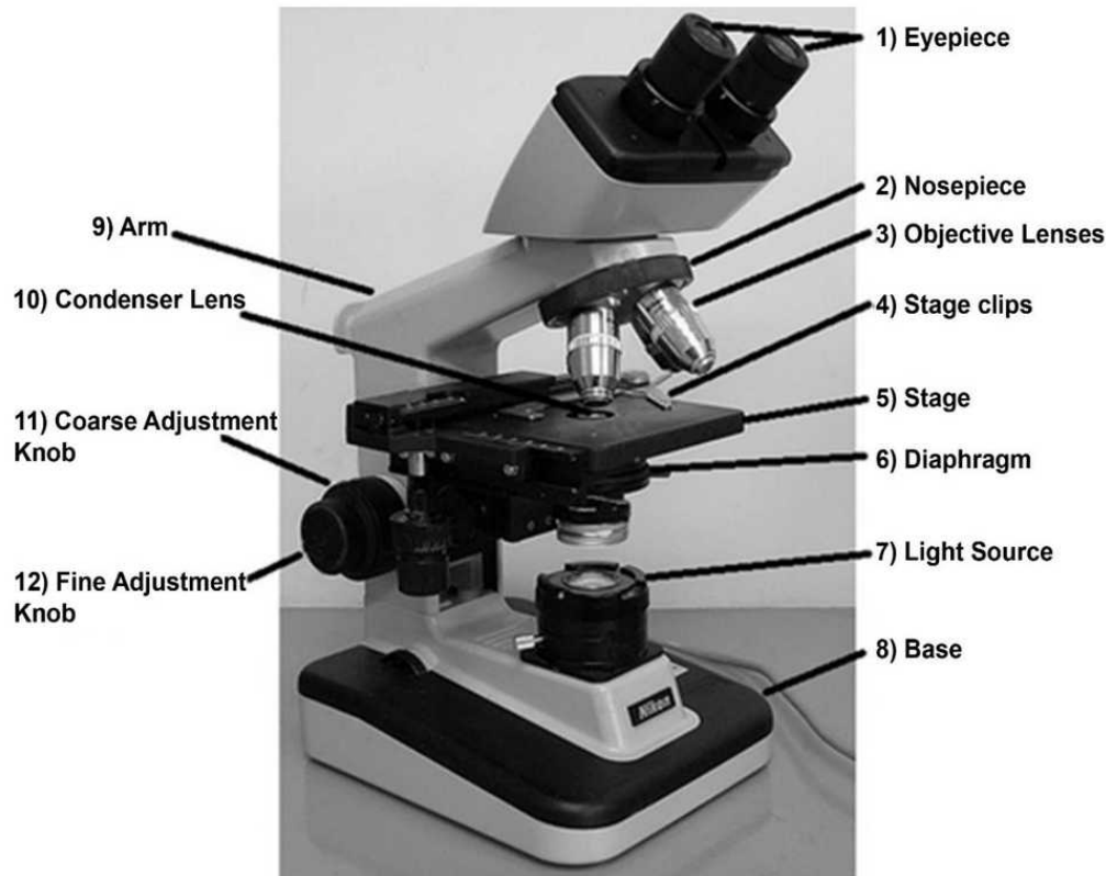
Figure 74.1 Parts of compound microscope
