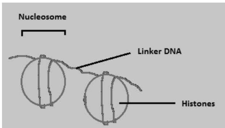
Figure 24.2 Two nucleosomes
