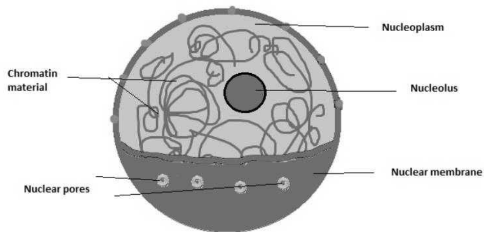
Figure 1.2 Organelle: Nucleus
