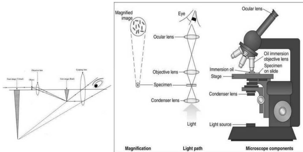
Figure 76.1 Compound/Bright-Field/Light Microscope
