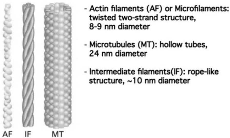
Figure 7.1 Cytoskeletal fibers
