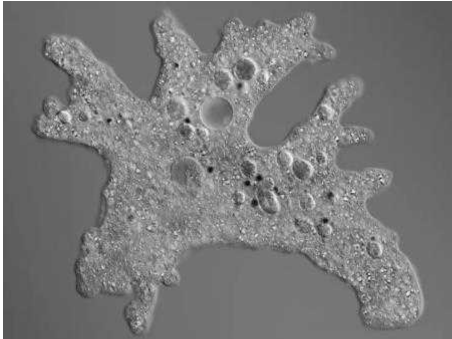
Figure 83.1 Amoeba
