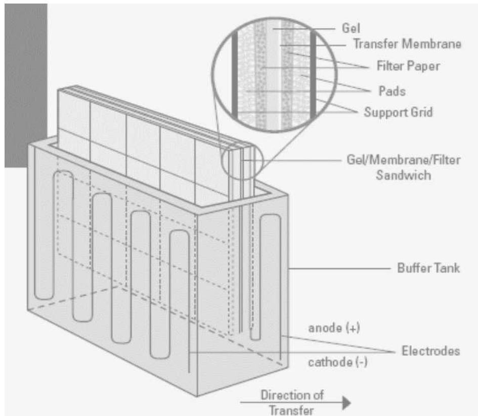
Figure 53.1 Electrophoretic transfer
