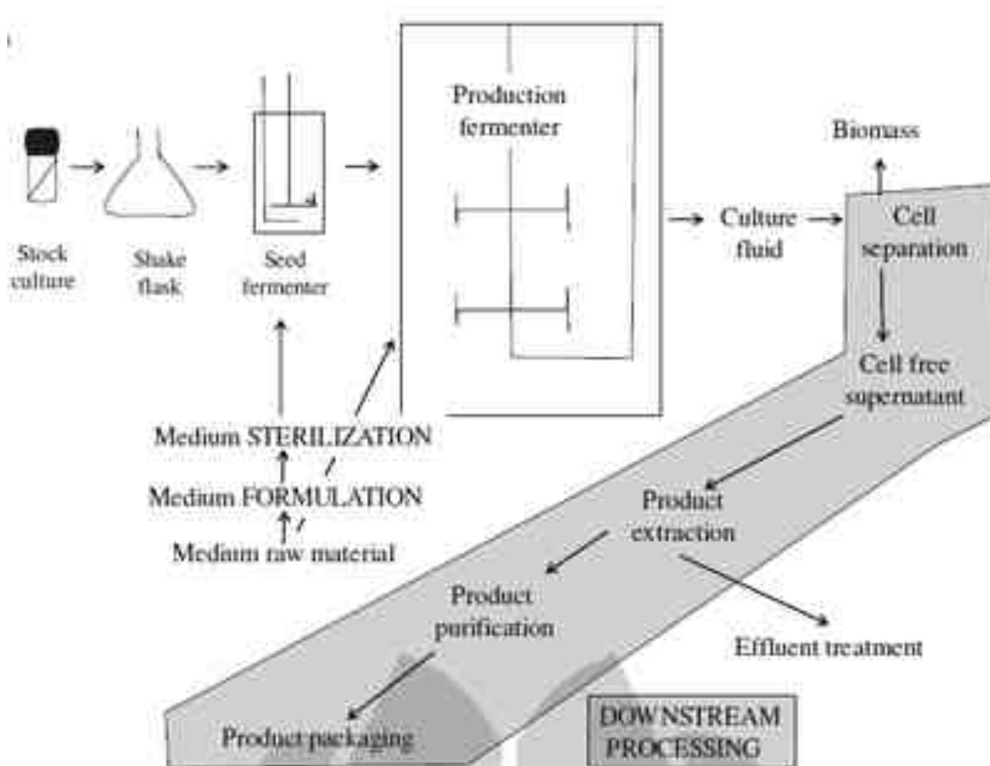
Flow sheet of a multipurpose fermenter and its auxiliary equipment
