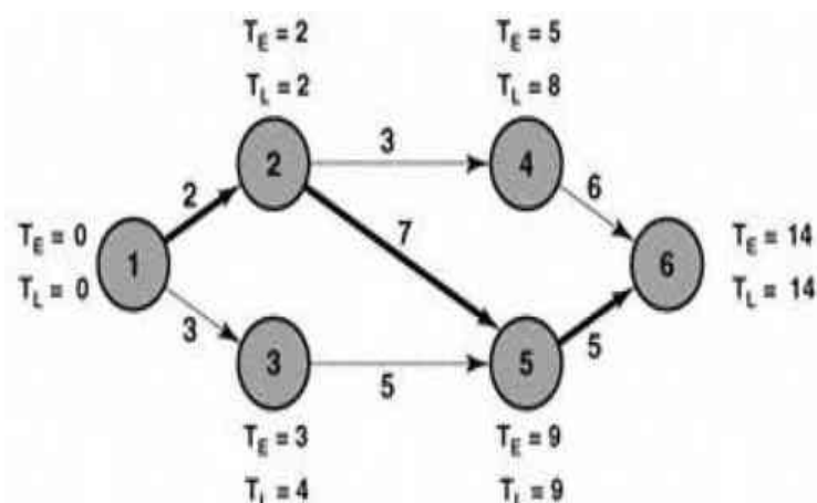
Figure 29.7: Network Replanning of Figure 29.1
