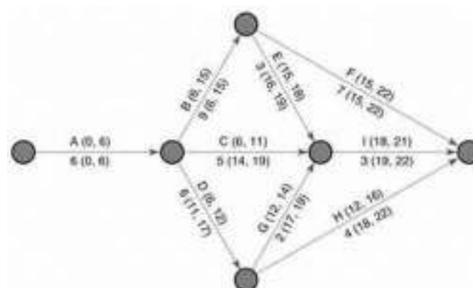
Figure 29.4: A Typical PERT Chart with Slack Times
