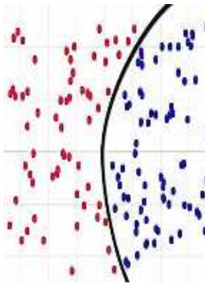
Classification
