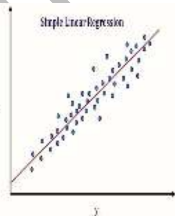
Regression
