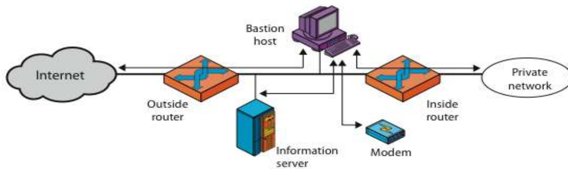
(c) Screened-subnet firewall system
