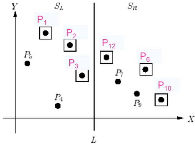
The maximal points of S_L and S_R
