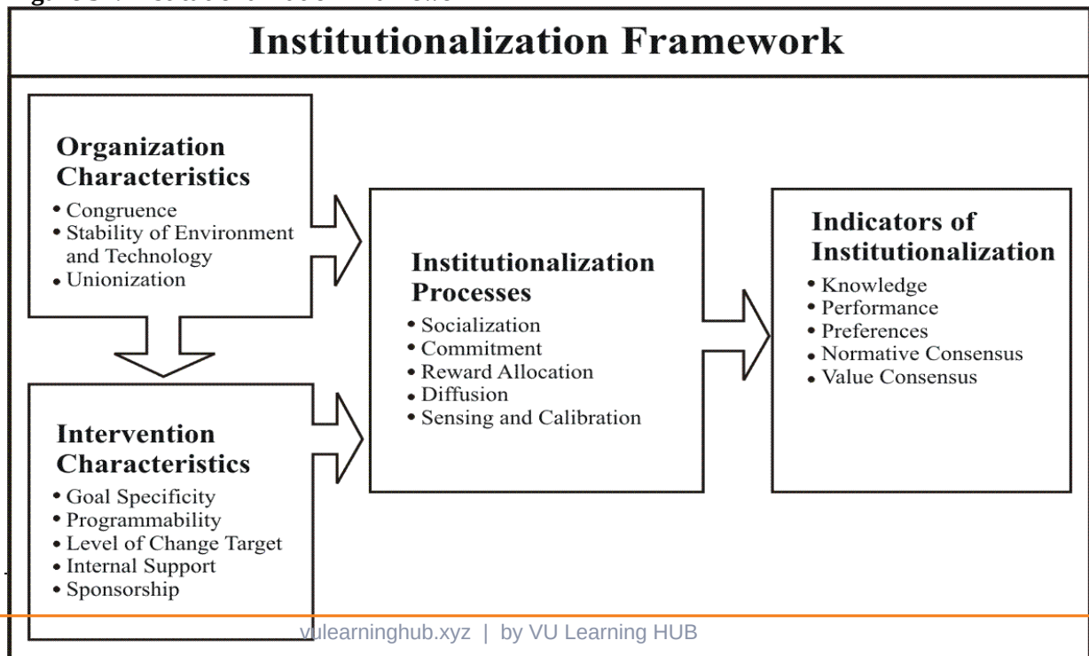
Figure 37: Institutionalization Framework
