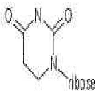
dihydrouridine
