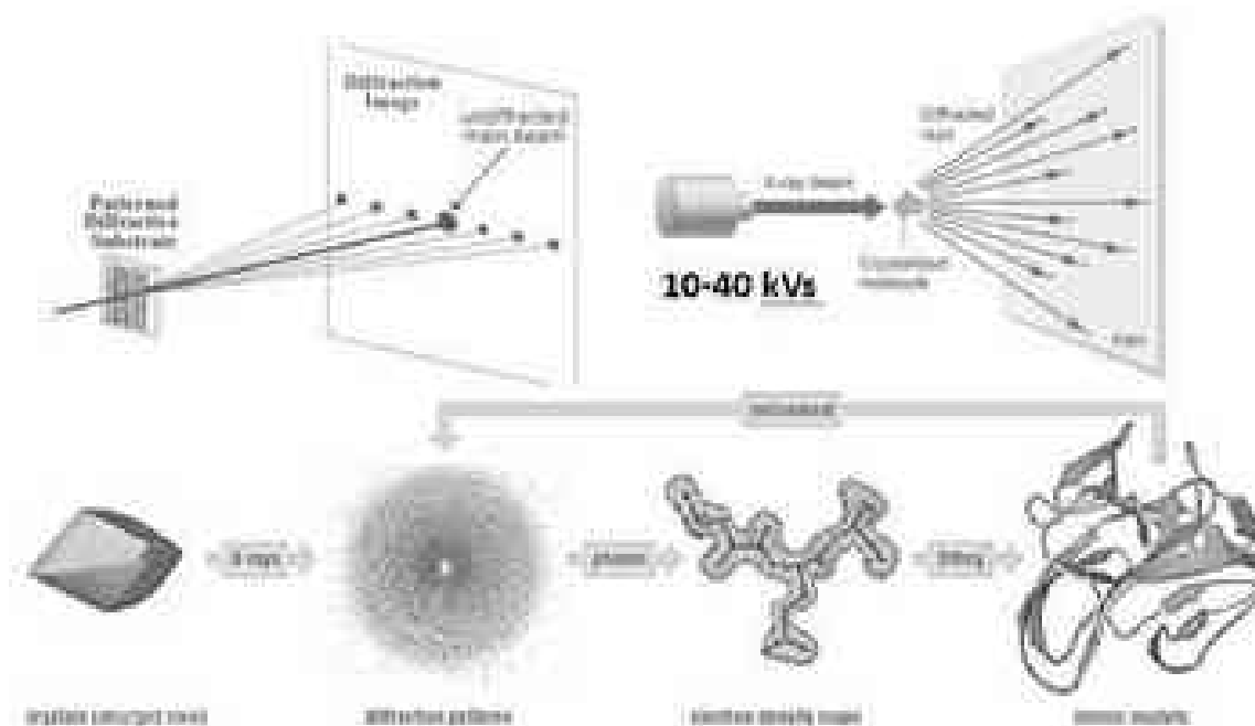
Figure 48 x-ray crystallography
