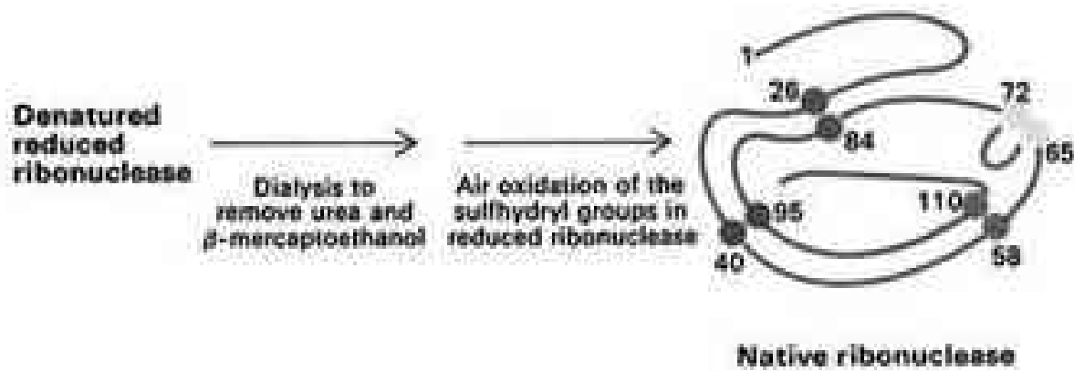
Figure 20 Anfinsen's Experiment
