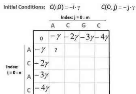
Figure 14 initial column and row are kept zero (0)
