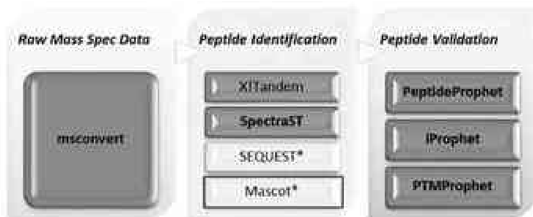
Figure 32 mzML http://tools.proteomecenter.org/software.php
