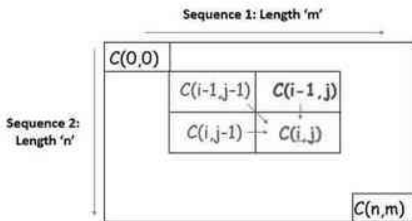
Figure 12 Needleman Wunsch algorithm way of computation of nucleotides
