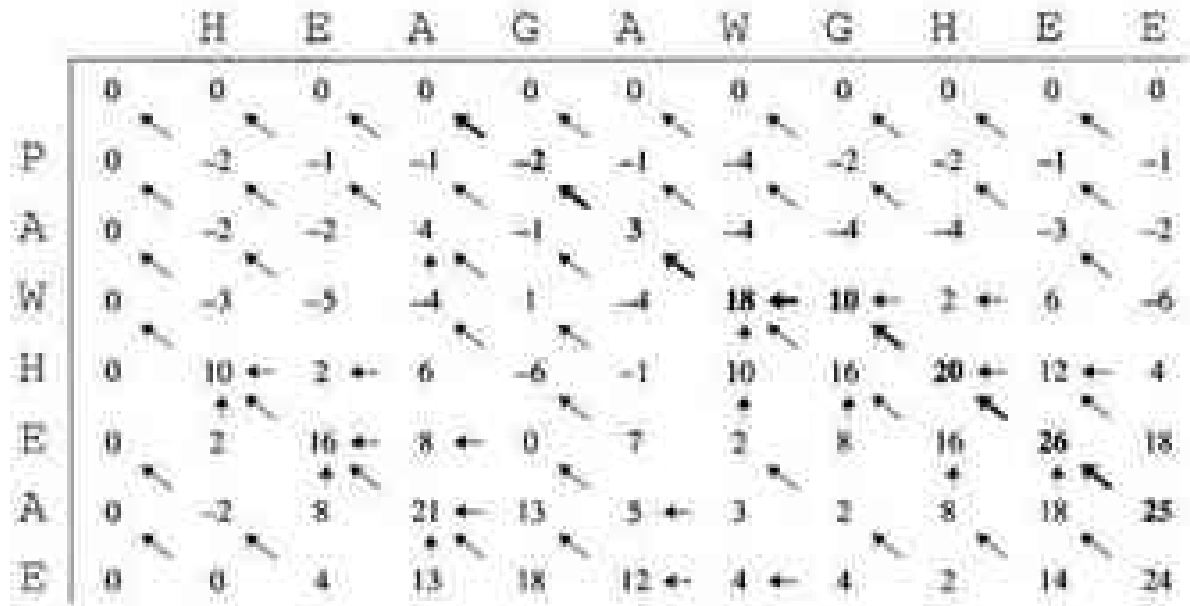
Figure 23 Traceback in amino acid sequence alignment
