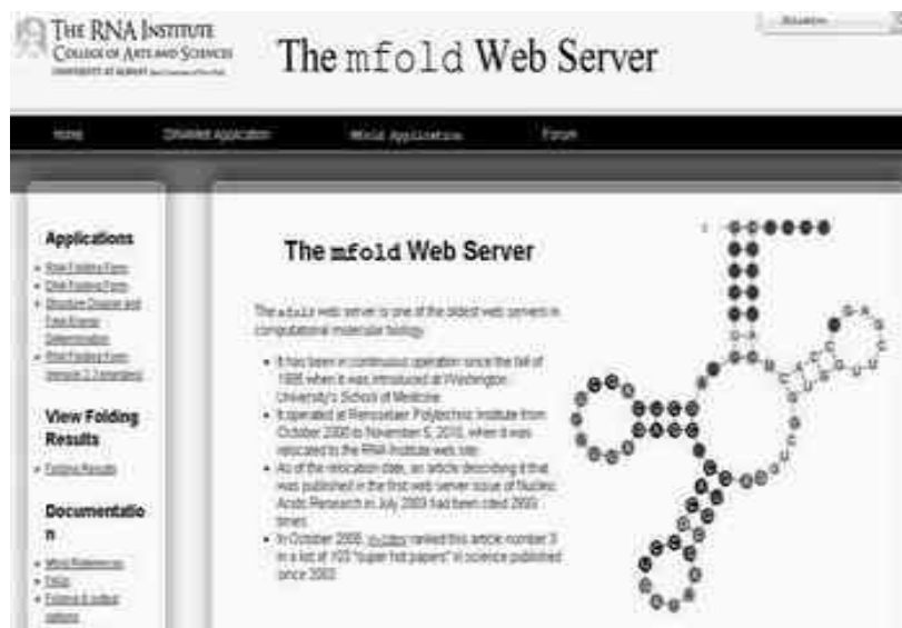
Figure 31 http://unafold.rna.albany.edu/?q=mfold
