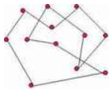
Polygon
