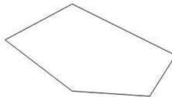
Convex Polygons
