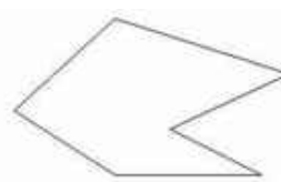
Simple Polygon
