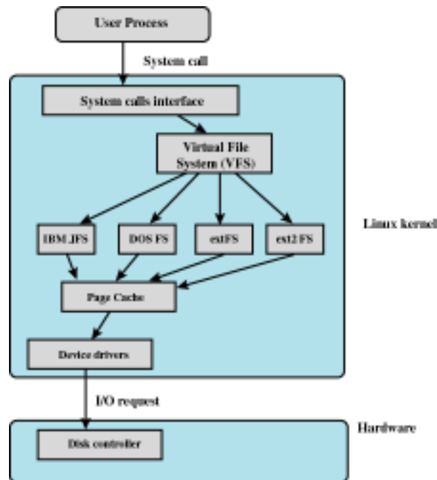
Linux Virtual File System Context
