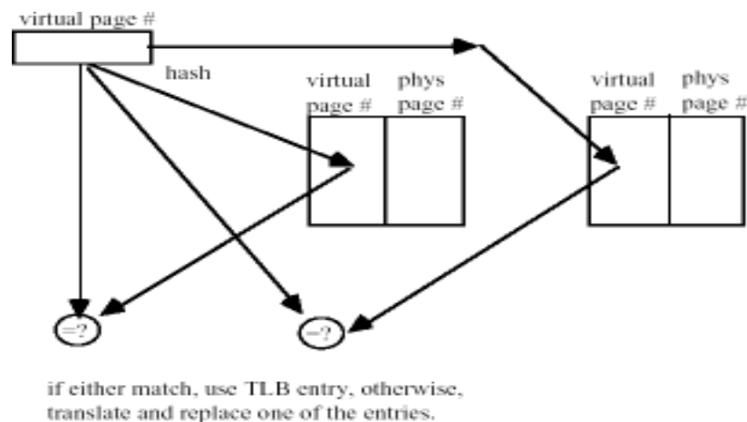
Two-way set associative
