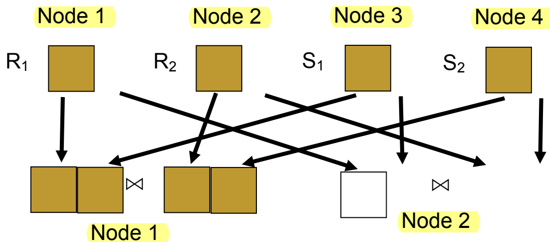
Figure 3: Parallel Hash Join (PHJ)
