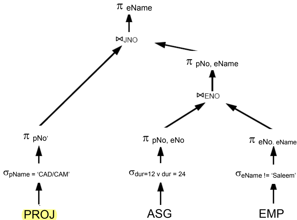
Figure 2: Rewritten operator tree
