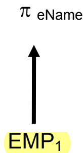
Generic query
