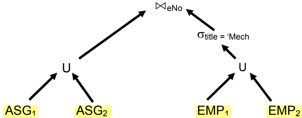
Generic query
