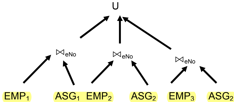
Figure 5: Reduced query
