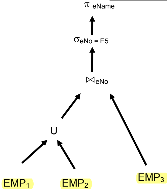
Figure 1: Generic query
