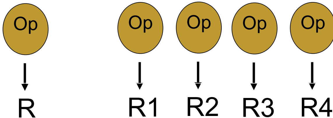
Figure 9: Intra-operator parallelism
