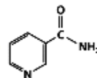
Nicotinamide
