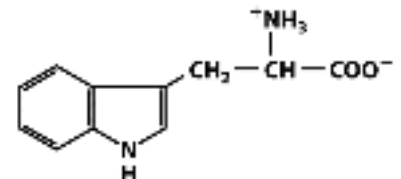
Tryptophan
