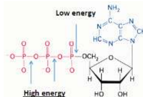
Adenosine Triphosphate
