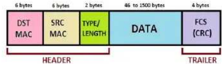
ETHERNET II (DIX) FRAME
