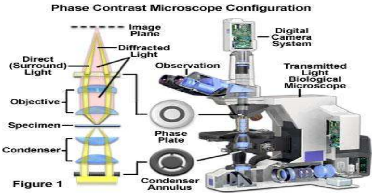
Figure 1 - Phase Contrast Microscope Configuration
