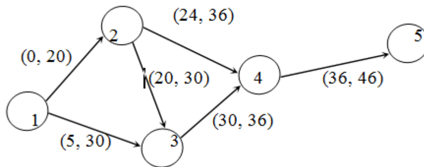
Late-Start Late-Finish Schedule Fig. 19
