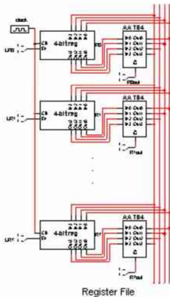
Multiple register connections
