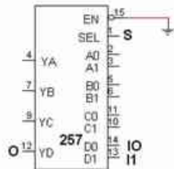
(b) TTL implementation domain
