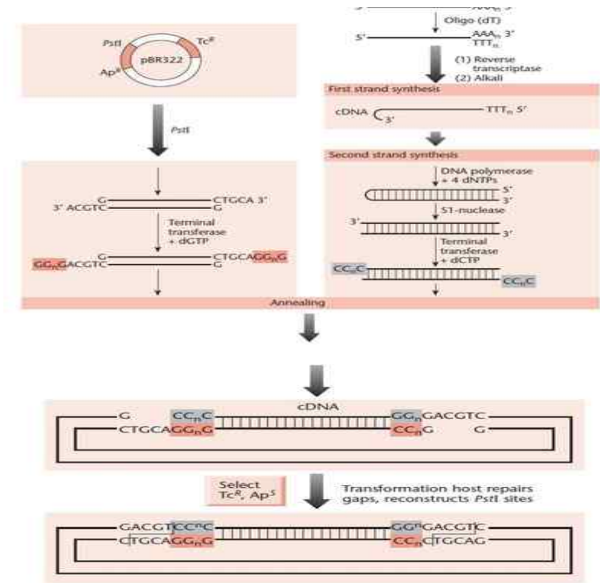
Fig: Insertion of cDNA into vector by homopolymer tailing
