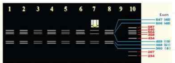
Fig. Results of multiplex PCR in a patient with Duchenne
