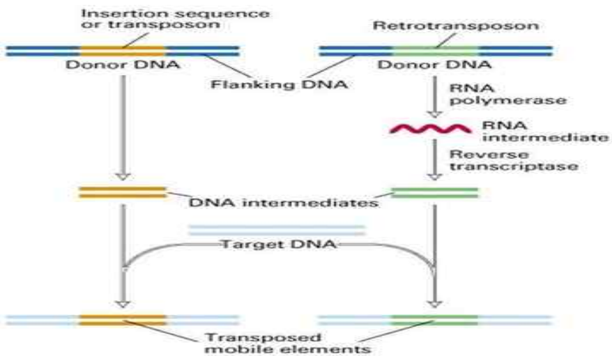
Retrotransposon moves using RNA intermediate (Figure)
