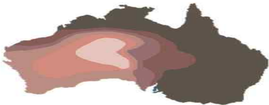
Frequency of Yellow-brown Hair
