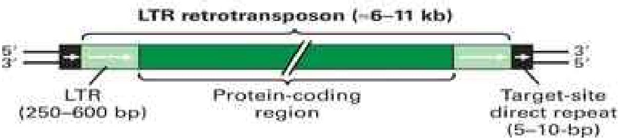
Long Terminal Repeats (Figure: a)
