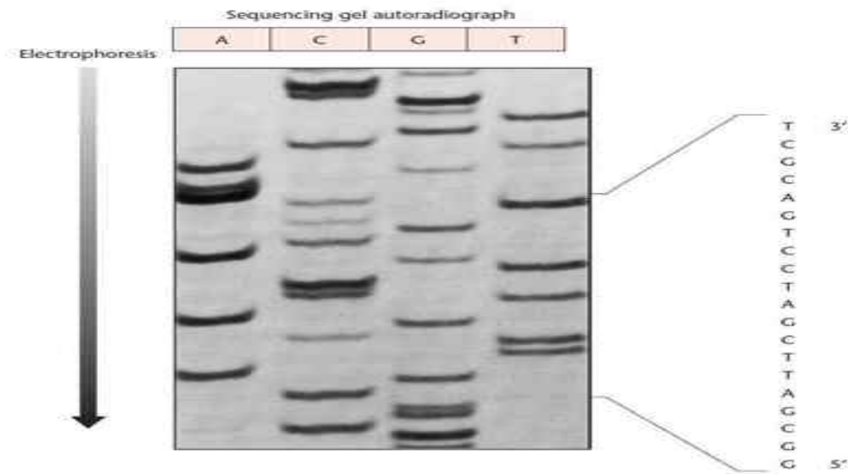
Fig: Autoradiograph of sequencing gel
