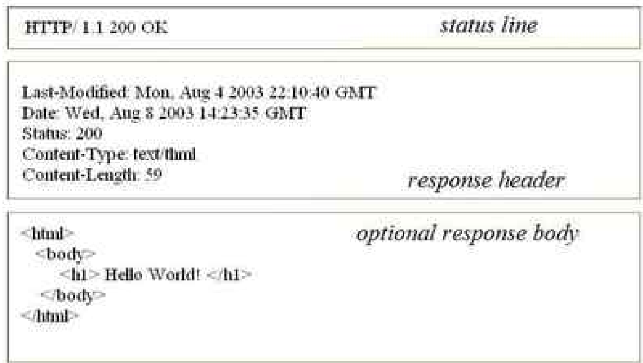
Figure 4: HTTP Response Example
