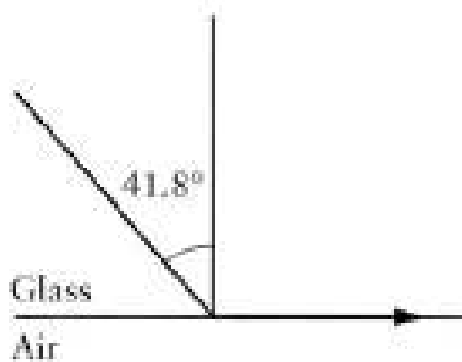
Figure 3: The critical angle.
