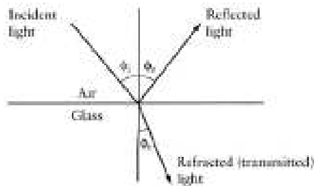
Figure 1: Light being reflected and refracted through a boundary.
