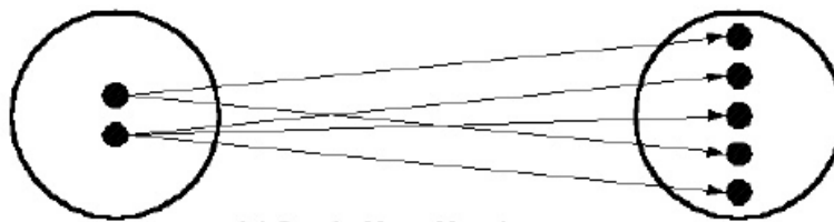
(c) One-to-Many Mapping
